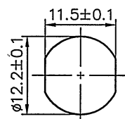
Panel Mounted
