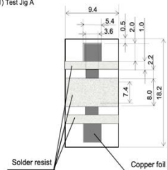
(1) Test Jig A
