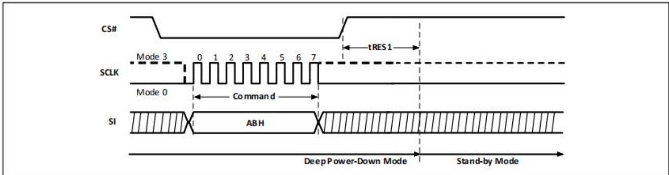
Figure-31. Read Electronic Signature (RES) Sequence Diagram
