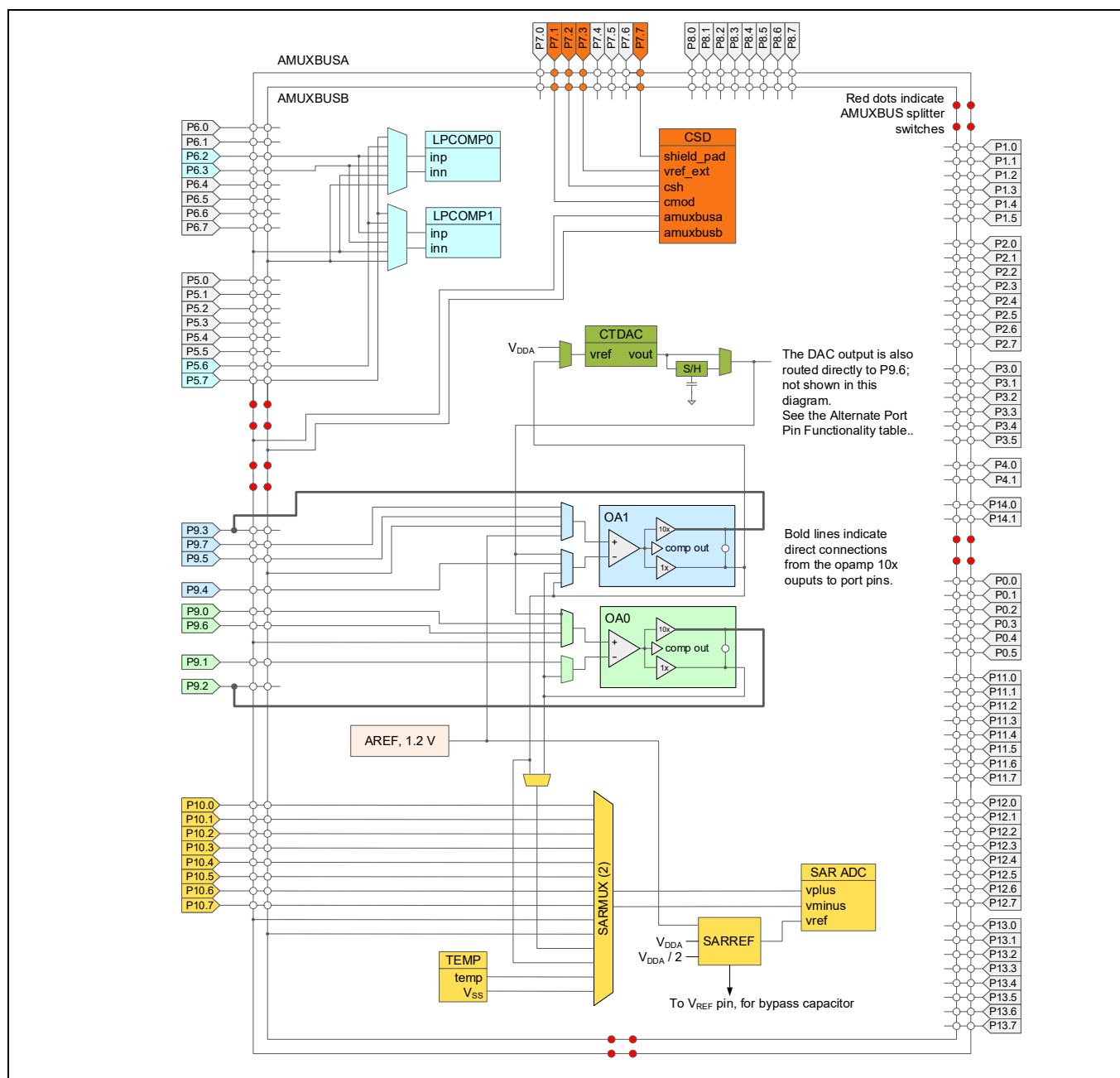
Figure 7 Analog subsystem
