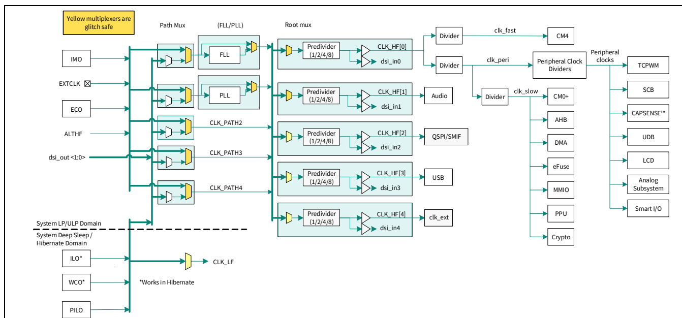
Figure 4 Clocking diagram
