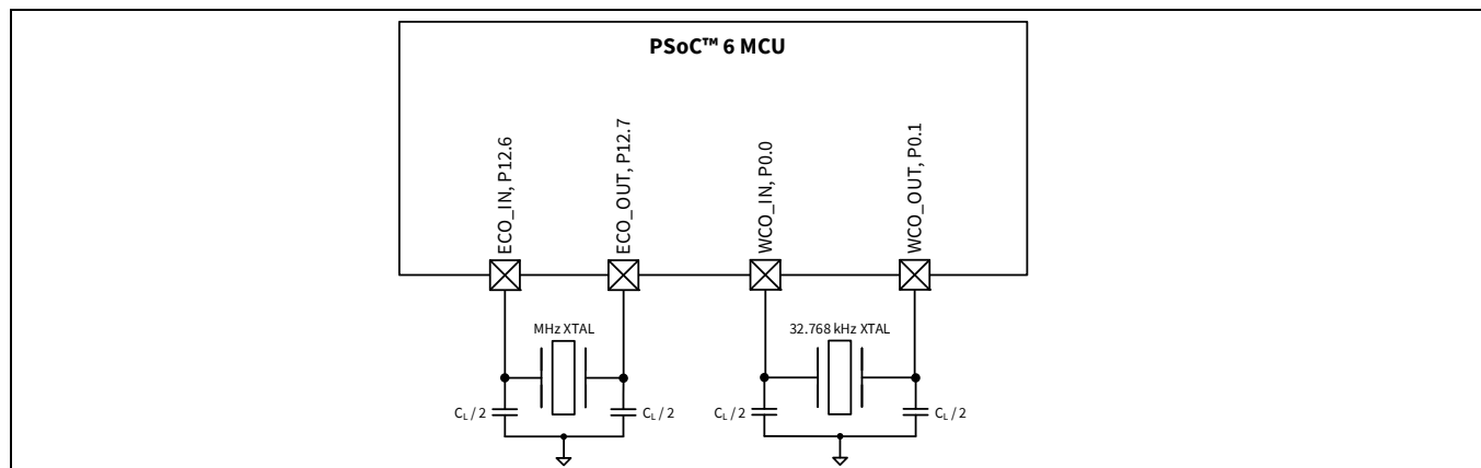
Figure 5 Oscillator circuits
