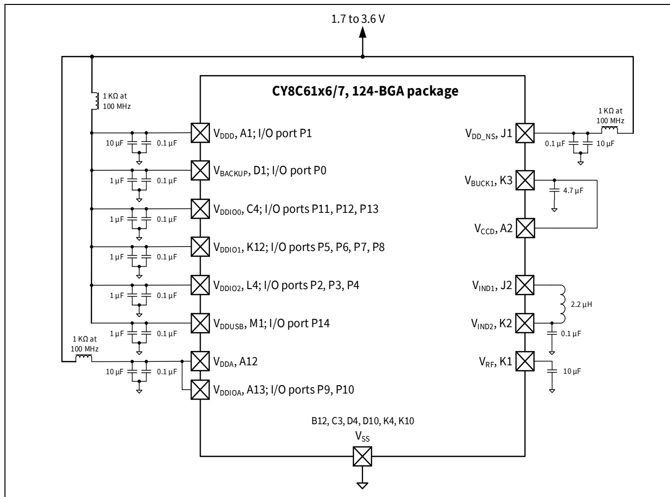
Figure 11 124-BGA power connection diagram
