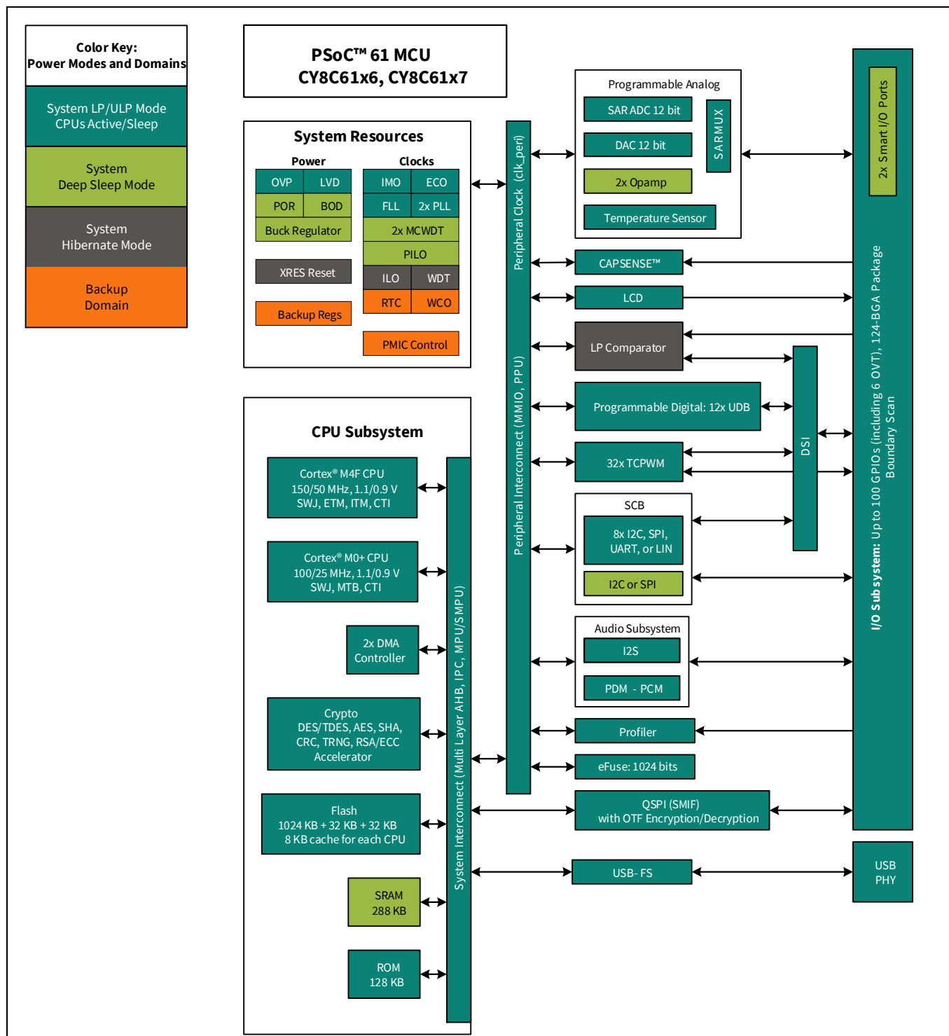
Figure 3 Block diagram
