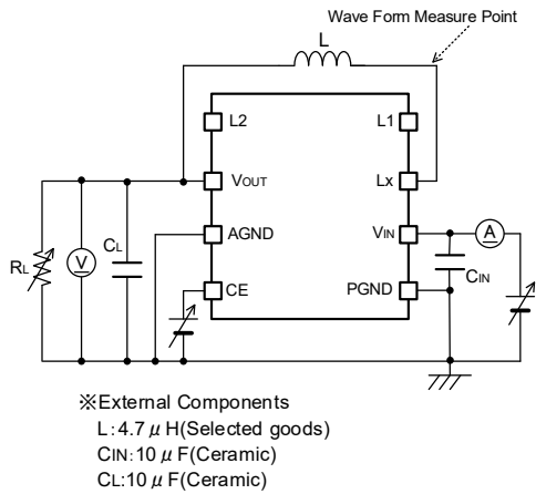
< Circuit No.③ >
