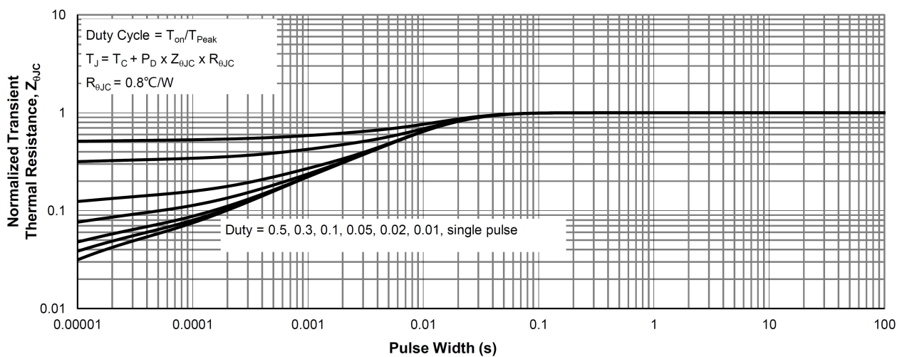
Normalized Transient Thermal Impedance
