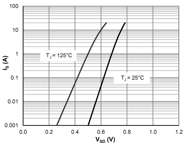
Body-Diode Characteristics
