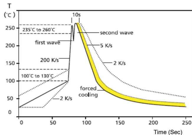
建議 double-wave Soldering Profile
