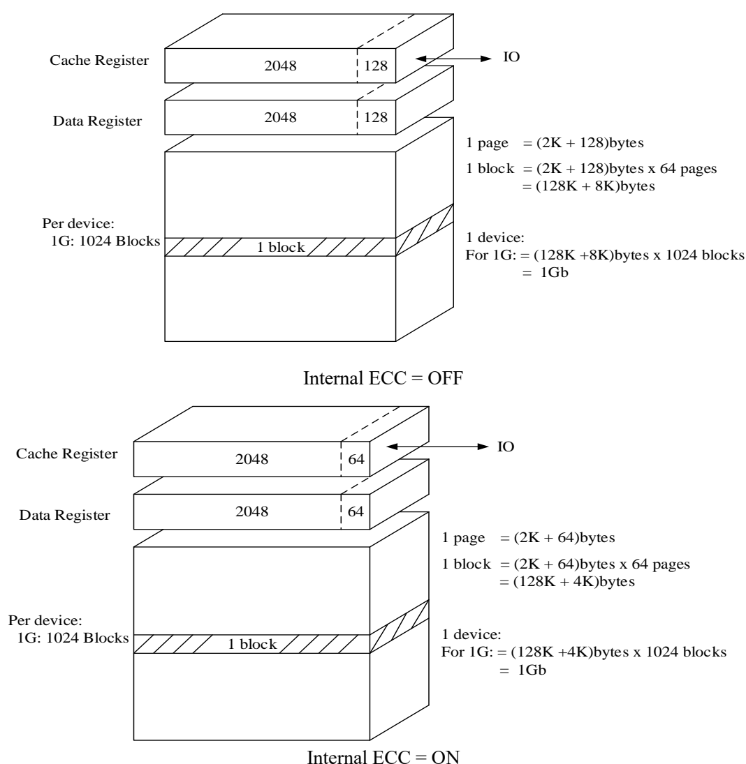
Figure 3. Array Organization
