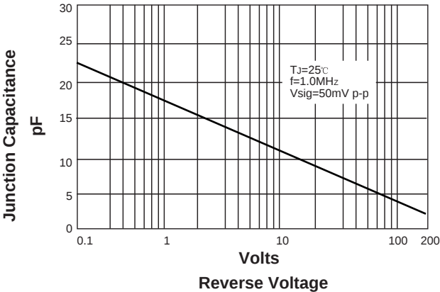
FIG. 5-TYPICAL JUNCTION CAPACITANCE
