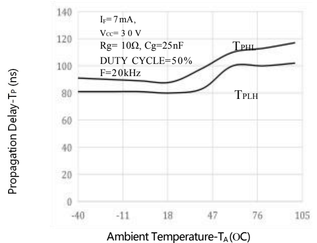
Fig.10 Propagation Delay vs Ambient Temperature
