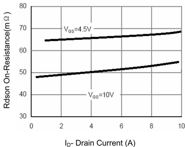
Figure 6 Drain-Source On-Resistance
