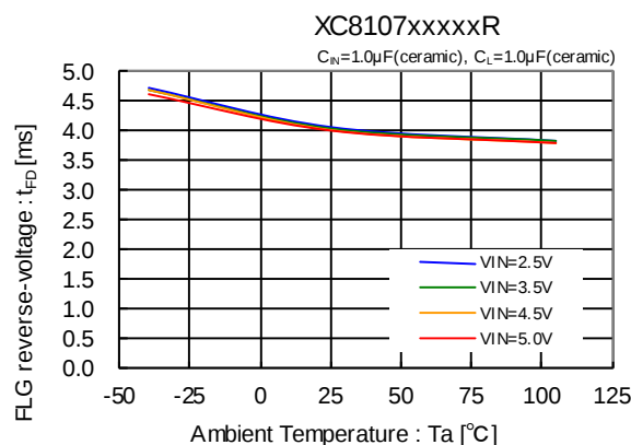
(22) FLG delay time reverse-voltage vs. Ambient Temperature
