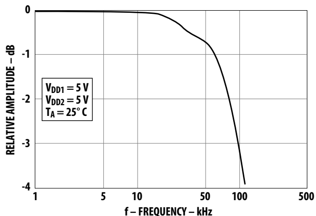
Figure 20 Amplitude Response vs. Frequency
