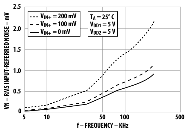
Figure 22 RMS Input-Referred Noise vs. Recommended Application Circuit Bandwidth
