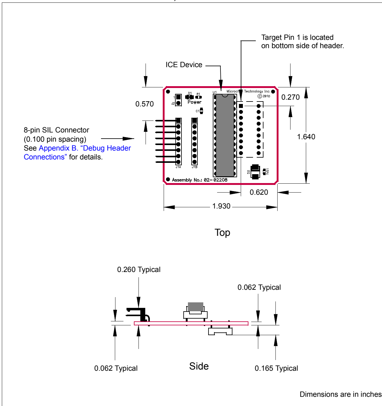
FIGURE 3-14: DIMENSIONS - AC244043, AC244044
