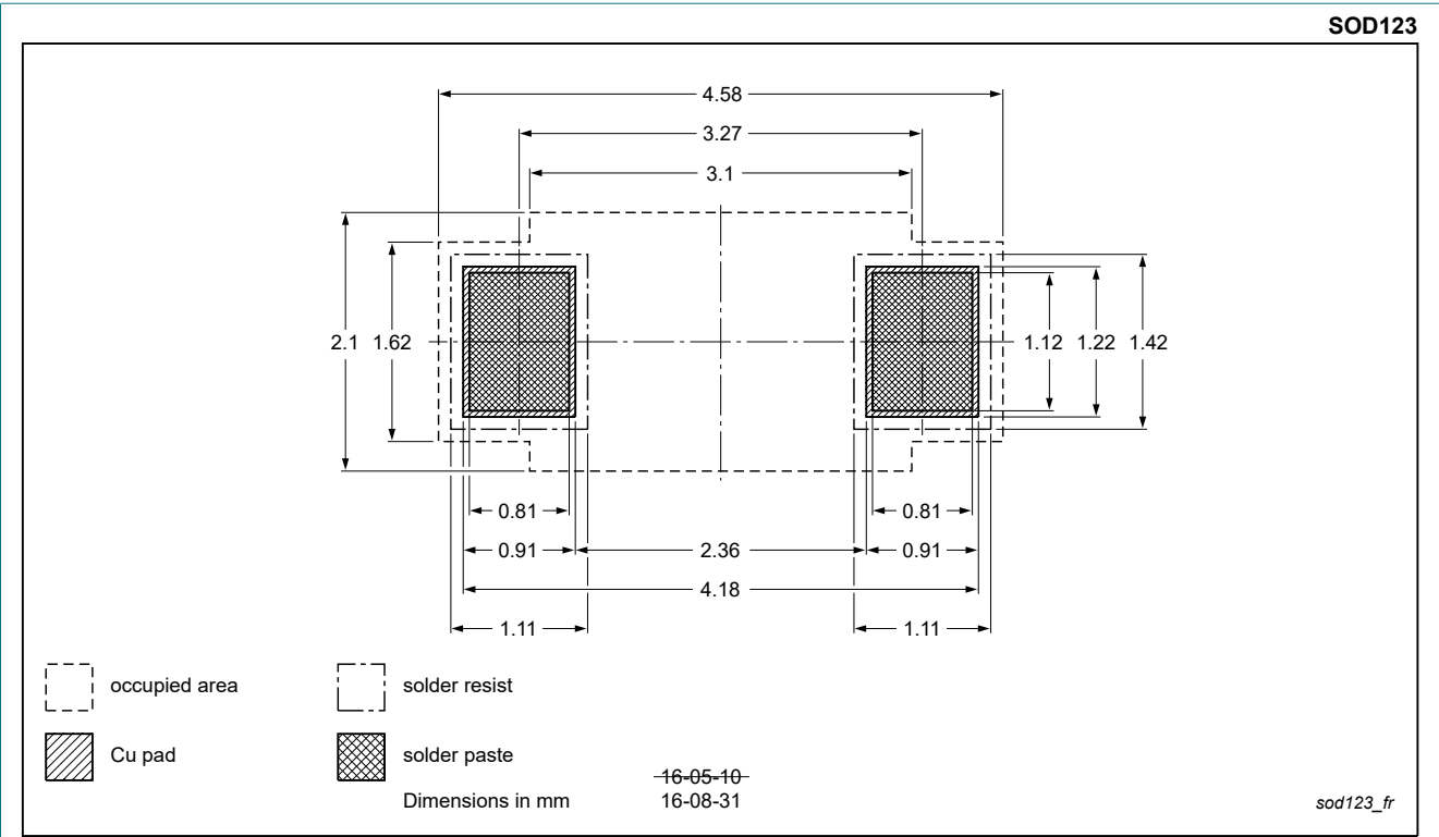
Fig. 9. Reflow soldering footprint SOD123
