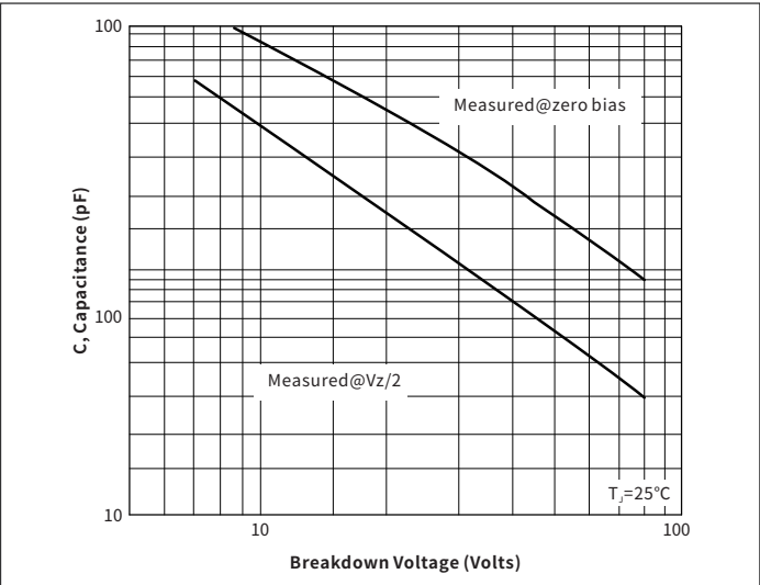
Fig.5 Typical Capacitance
