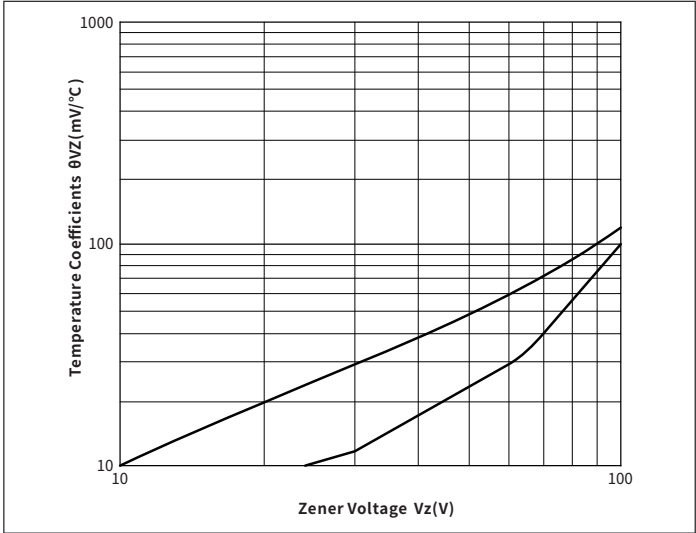
Fig.4 Temperature Coefficient
