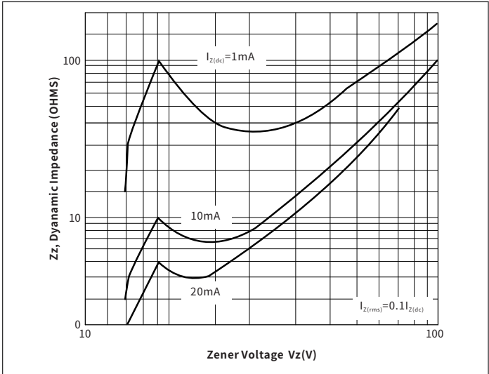
Fig.6 Effect of Zener Voltage on Zener Impedance
