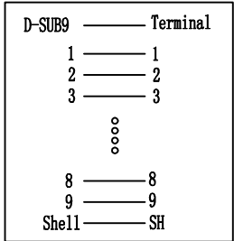
Pin assignment
