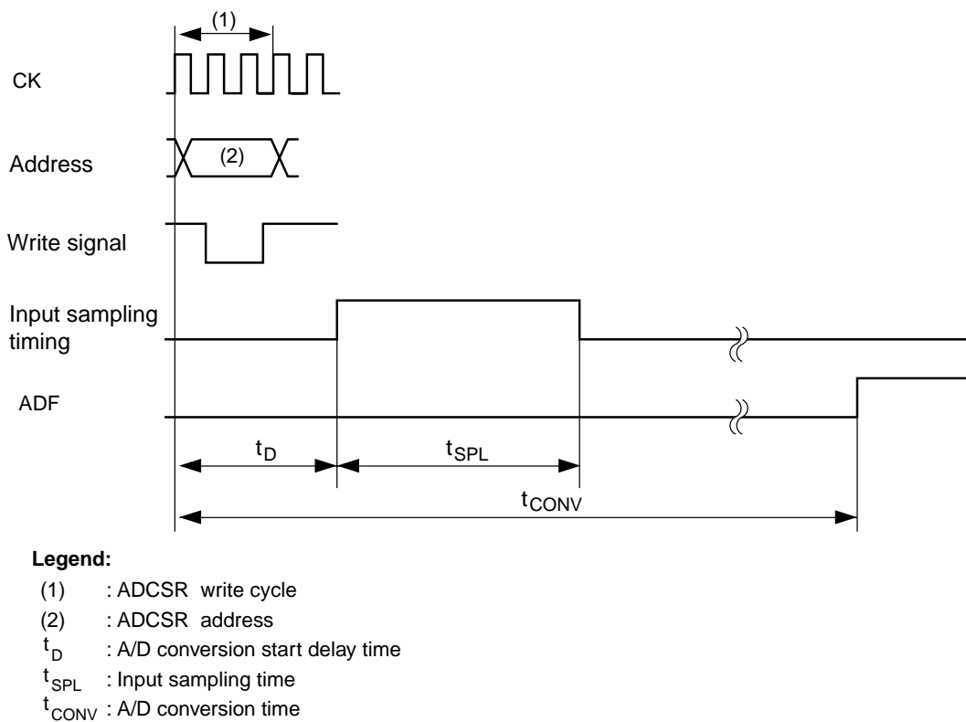
Figure 26.32 Analog Conversion Timing
