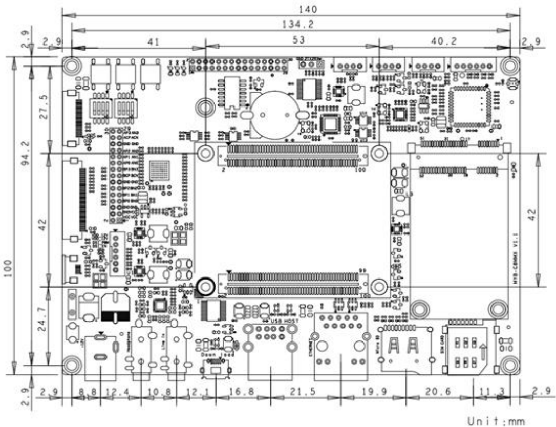
Figure 1-11 MYD-C8MMX-V2 Dimensions Chart
