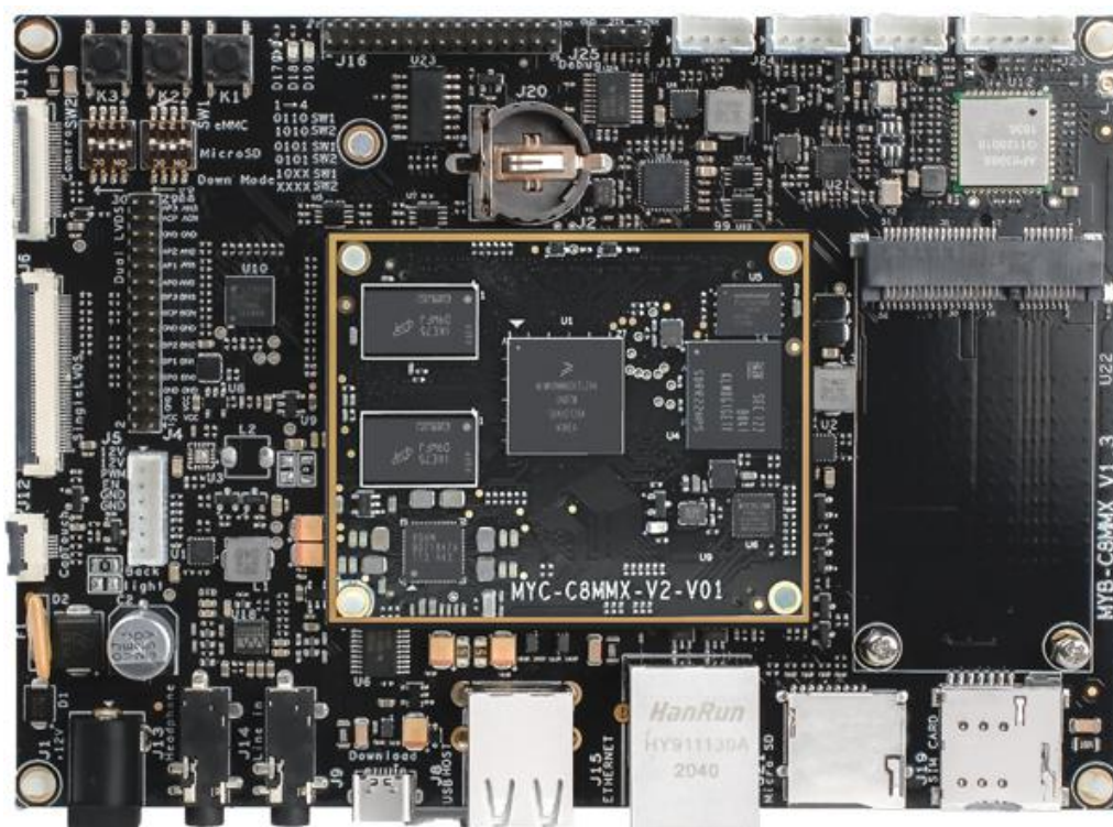
Figure 1-1 MYD-C8MMX-V2 Development Board
