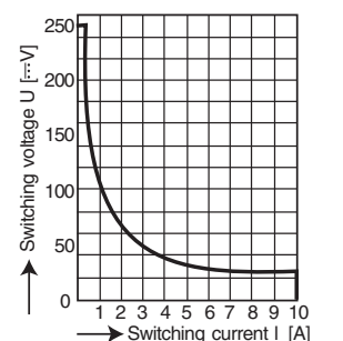
Maximum switching power curve
