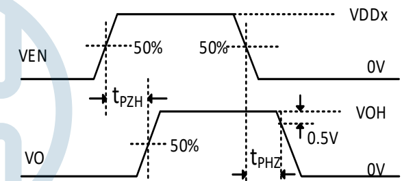
Figure 14. t_{PZH}/t_{PHZ} measurement waveform
