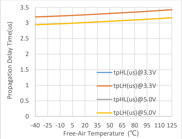
Figure 7.π13xU3x Propagation Delay Time vs. Free-Air Temperature
