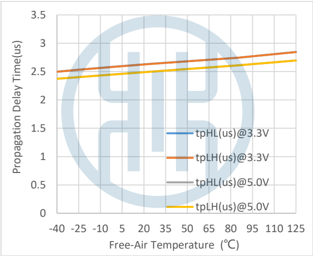
Figure 8.π13xU6x Propagation Delay Time vs. Free-Air Temperature
