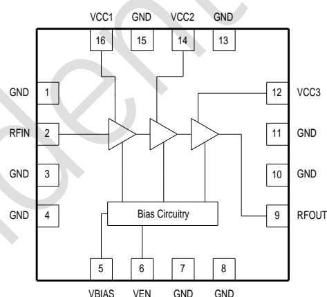
Figure 2. GDM0628 Function Block Diagram
