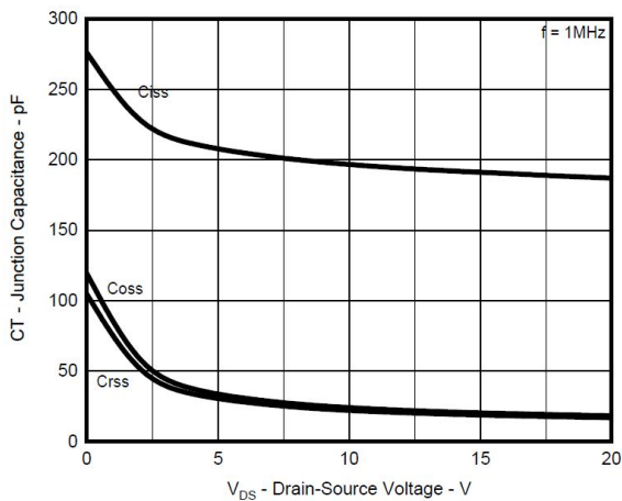
Fig.5 Capacitance Characteristics
