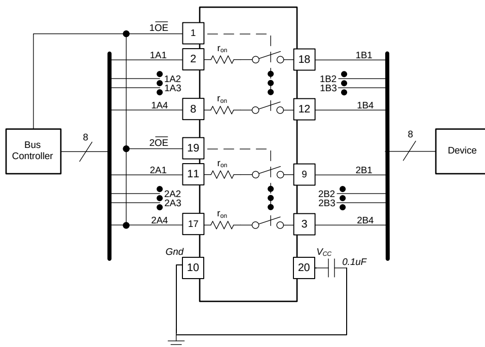
Figure 4. Typical Application
