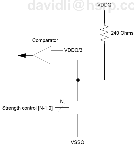
Figure 21. pull-down calibration
