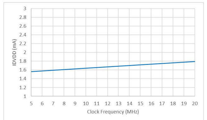
Figure 5.24 Digital Side Supply Current vs Clock Frequency
