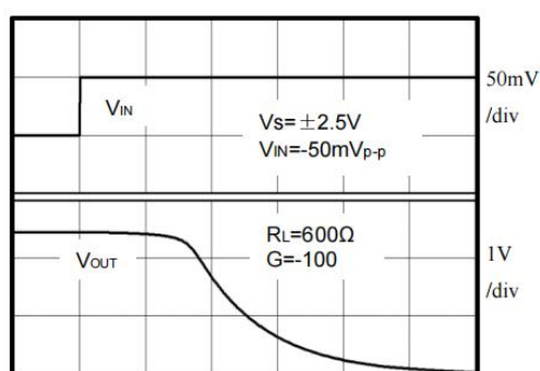
Positive Overload Recovery
