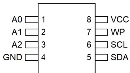
SOP-8/DIP-8/MSOP-8
