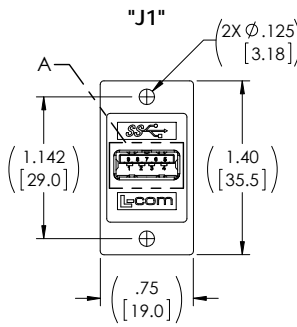
USB3.0 SERIES "A" RECEPTACLE BULKHEAD ADAPTOR CONTACTS: 30 μINCHES GOLD PLATING
