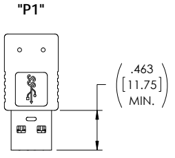
USB3.0 SERIES "A" PLUG DOWN EXIT CONTACTS: 30 μINCHES GOLD PLATING
