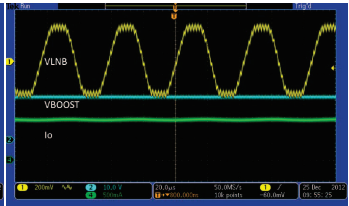
Figure 34. V_{IN} = 5\text{ V} , V_{LNB} = 18.6\text{ V} , 0.5 A, 22-kHz Tone
