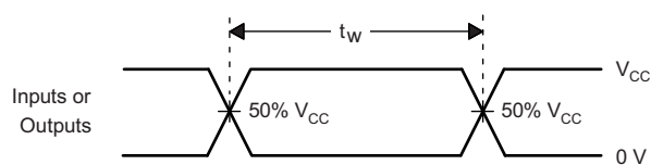
Figure 7. Voltage Waveforms Pulse Duration
