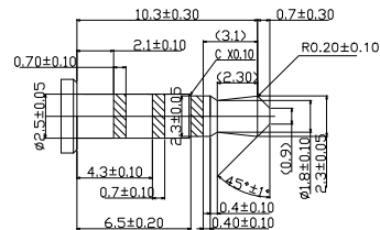
(ø2.50mm 4 POLE PLUG DETAIL DRAWING)
