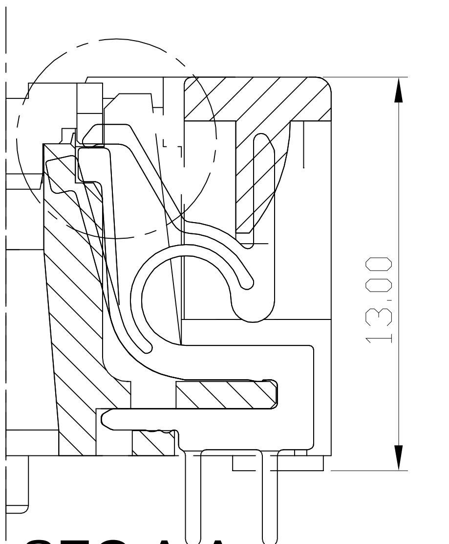
SEC.A-A Contact Retracted
