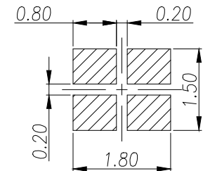
METAL MASK T=0.10 TOLERANCE ±0.05 (銅網公差)
