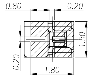
RECOMMENDED PCB LAYOUT TOLERANCE ±0.05 (銅箔公差)
