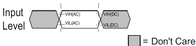
Figure 3. LPDDR4 Input AC timing definition for CKE 1-1). AC level is guaranteed transition point. 1-2). DC level is hysteresis.
