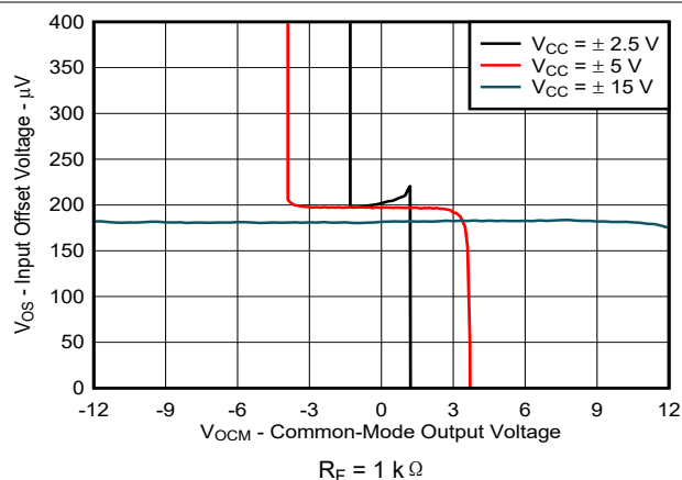
图 7-26. Input Offset Voltage vs Common-Mode Output Voltage
