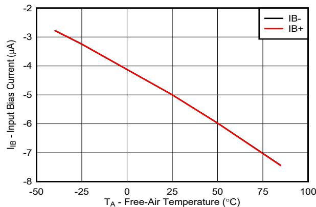
图 7-11. Input Bias Current vs Free-Air Temperature
