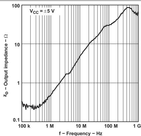
图 7-56. Output Impedance vs Frequency
