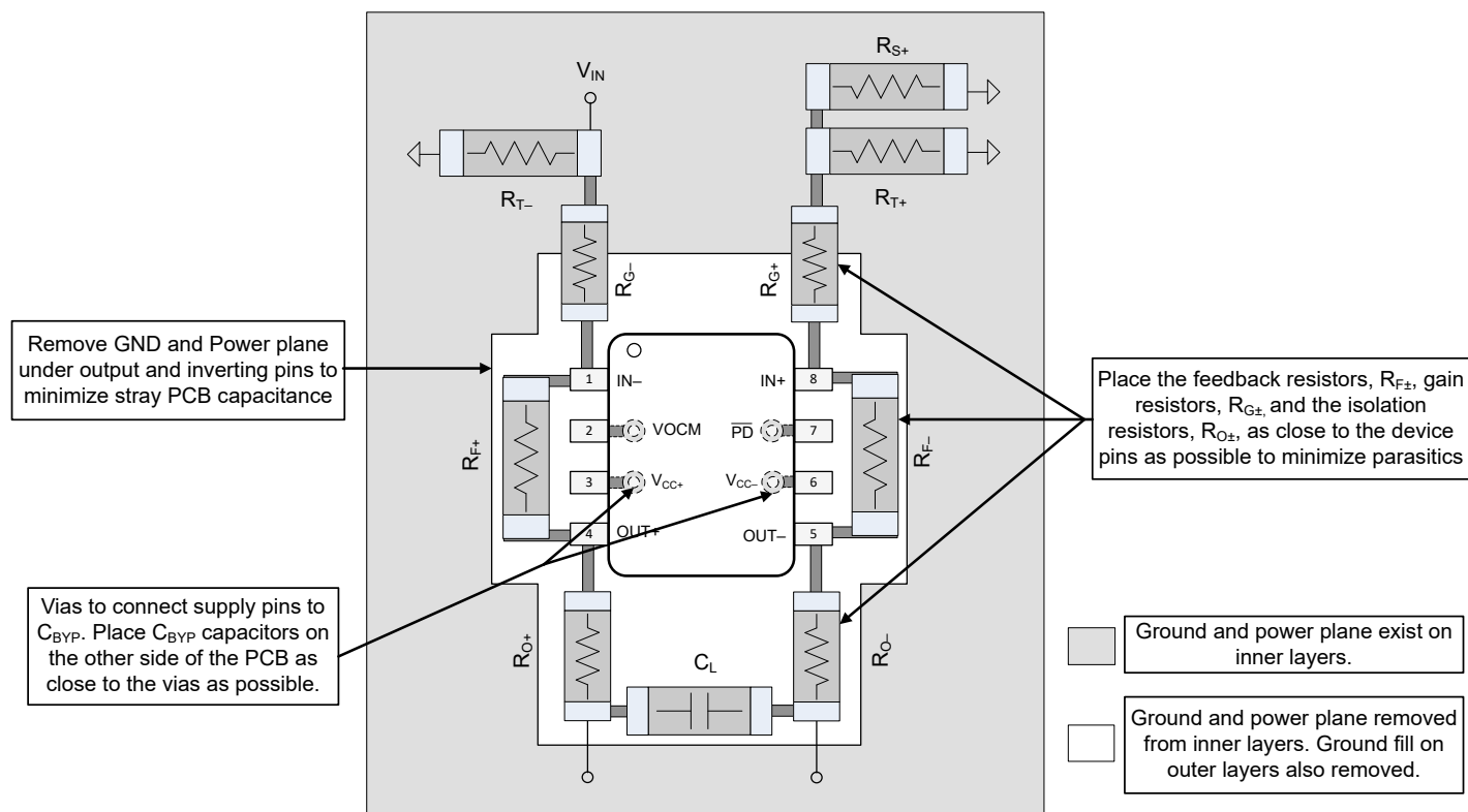
图 11-2. Layout Recommendations
