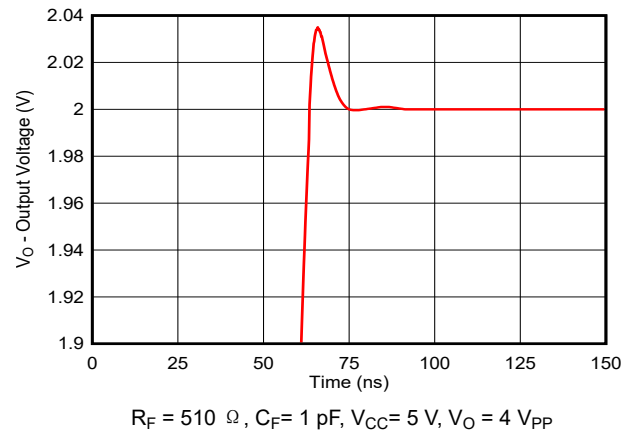
图 7-12. Settling Time
