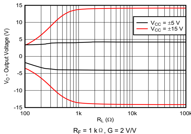
图 7-27. Output Voltage vs Differential Load Resistance
