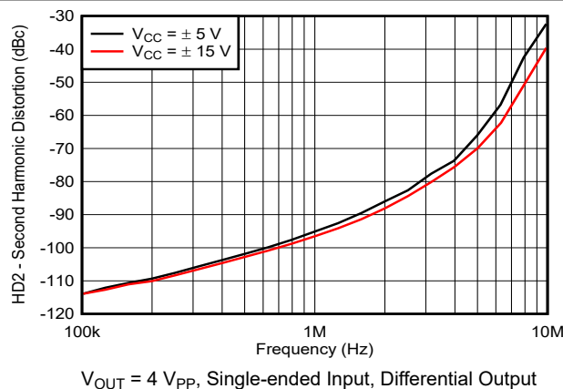
图 7-17. Second-Harmonic Distortion vs Frequency
