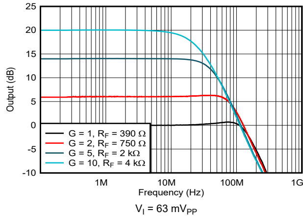
图 7-1. Small-Signal Frequency Response
