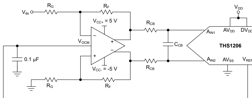
图 9-2. Fully-Differential Amplifier Attached to a Differential ADC
