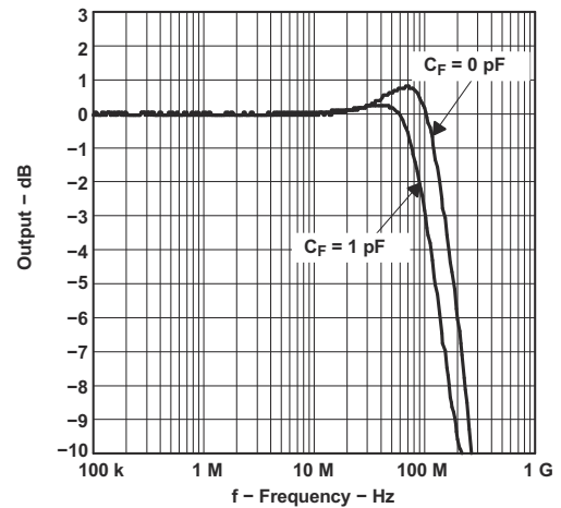
图 7-32. Small-Signal Frequency Response (Various CF)
