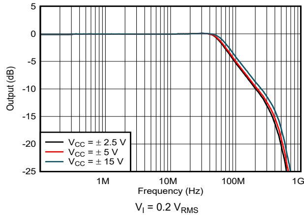
图 7-7. Large-Signal Frequency Response
