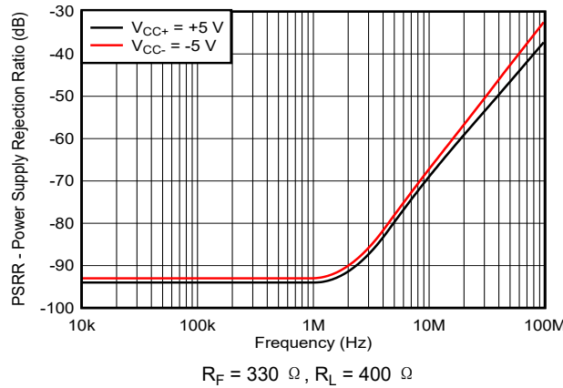
图 7-13. Power-Supply Rejection Ratio vs Frequency (Differential Out)
