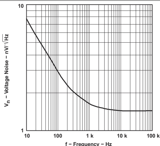
图 7-52. Voltage Noise vs Frequency
