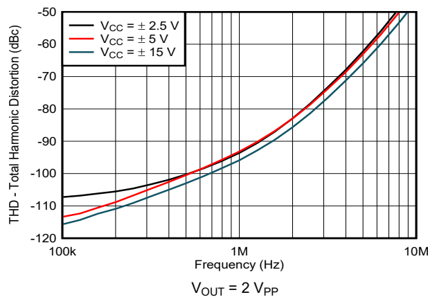
图 7-15. Total Harmonic Distortion vs Frequency
