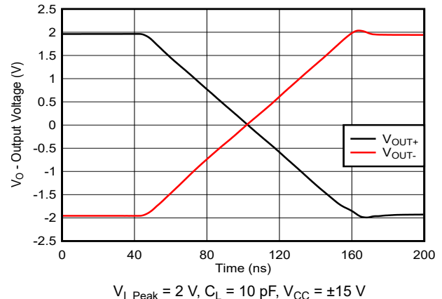
图 7-14. Large-Signal Transient Response
