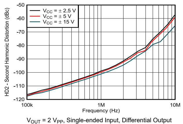
图 7-16. Second-Harmonic Distortion vs Frequency
