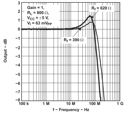
图 7-30. Small-Signal Frequency Response
