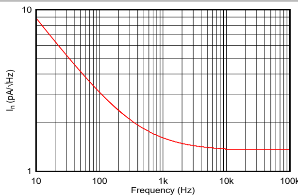
图 7-25. Current Noise vs Frequency
