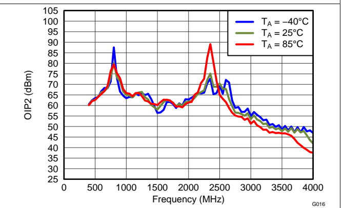
Figure 17. OIP2 vs LO Frequency ( f_{LO} ) and Temperature
