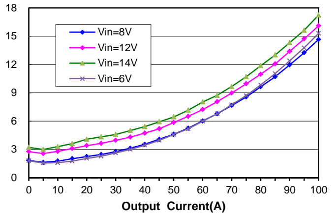
Power Dissipation vs. Load Current
