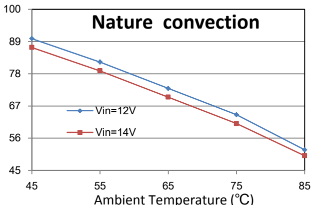
Ambient Temperature vs. Load Current
