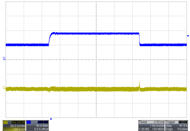
Transient Response V_{IN}=12V , Step from 50A-90A~50A Blue: Output Current Yellow: Output Ripple
