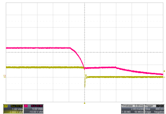
Shut-down V_{IN}=12V , I_O=100A Red: Input Voltage Yellow: Output Voltage
