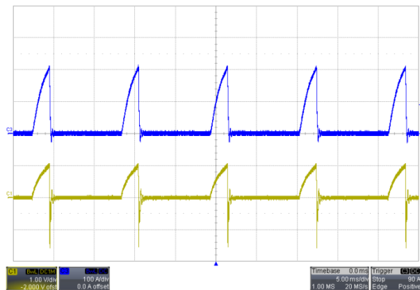
Short-Circuit Output V_{IN}=12V
