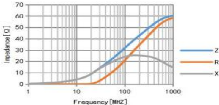
产品特性曲线图：Product Characteristic Curve
