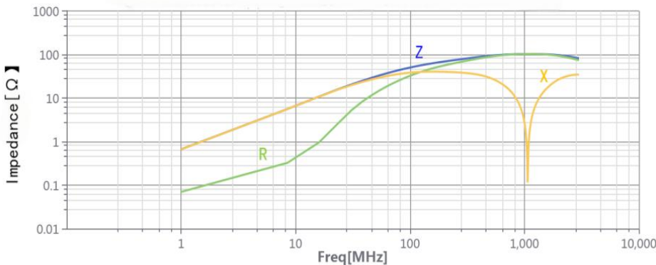
产品特性曲线图：Product Characteristic Curve
