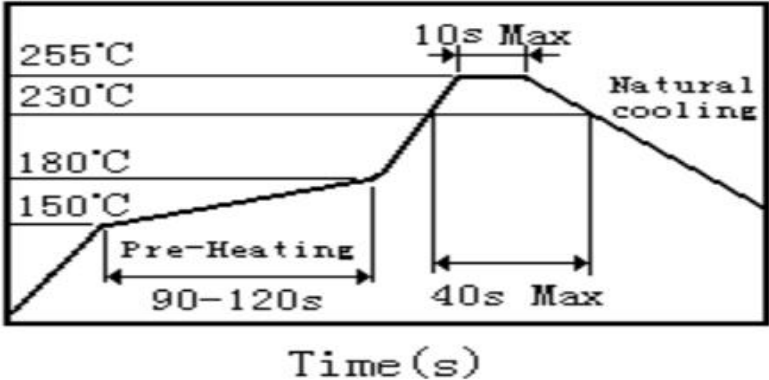
回流焊曲线 Reflow soldering profile
