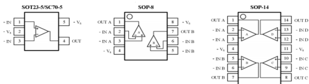
Figure 1 Pin Configurations
