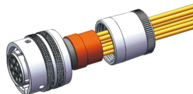
STEP3: ALIGN THE CONTACTS INTO THEIR CORRESPONDING INSERT HOLES. THEN SLIDE THE GROMMET UP THE WIRES CLOSE TO INSERT.
