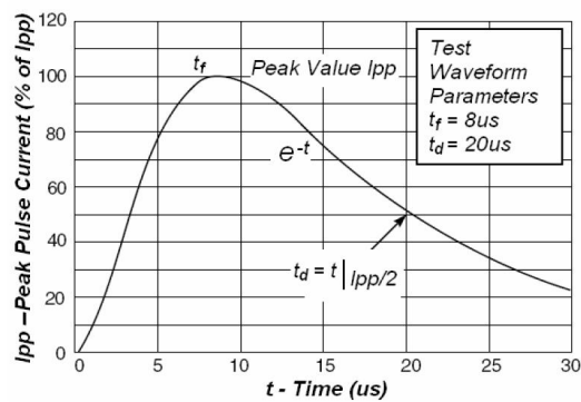
Fig3. Pulse Waveform
