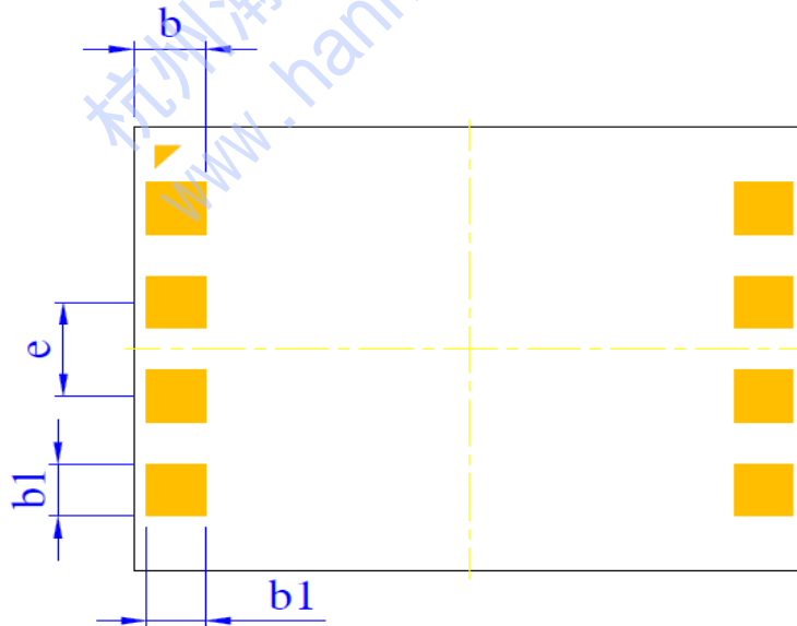
Figure 3: Bottom View
