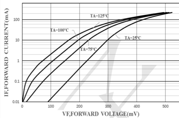
FIG 2.TYPICAL FORWARD CHARACTERISTIC
