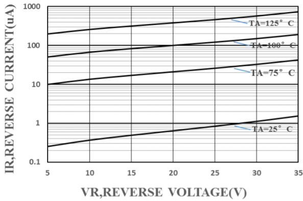
FIG 1.TYPICAL REVERSE CHARACTERISTIC
