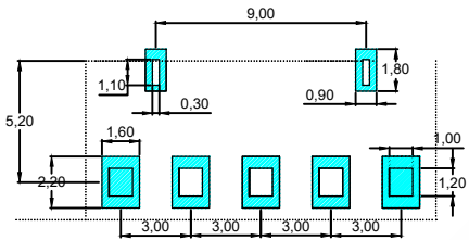
RECOMMENDED PCB LAYOUT TOP VIEW (. XX ± 0.05)
