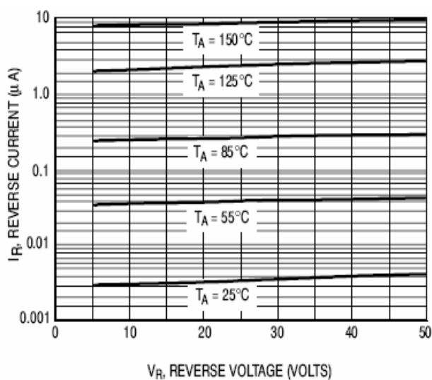
Figure 2. Leakage Current
