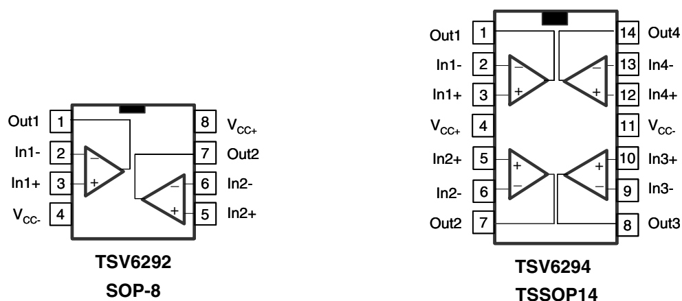
Figure 1. Pin connections for each package (top view)
