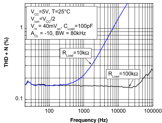
Figure 17. Distortion + noise vs. frequency at V_{CC} = 5\text{ V}
