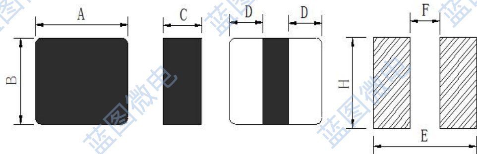
Recommended Land Pattern
